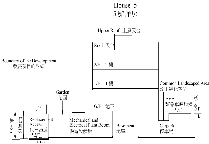
Cross-section Plan (8) 橫截面圖 (8)
