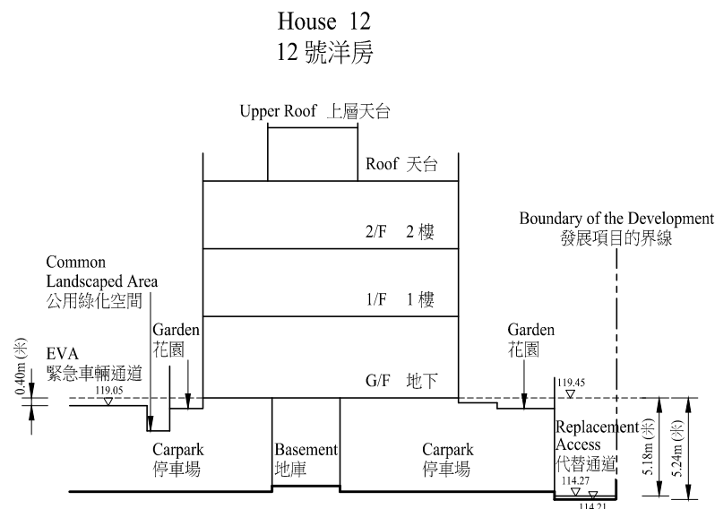
Cross-section Plan (15) 橫截面圖 (15)
