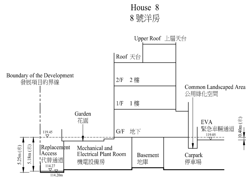
Cross-section Plan (11) 橫截面圖 (11)
