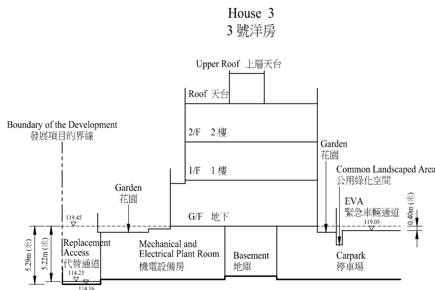
Cross-section Plan (7) 橫截面圖 (7)
